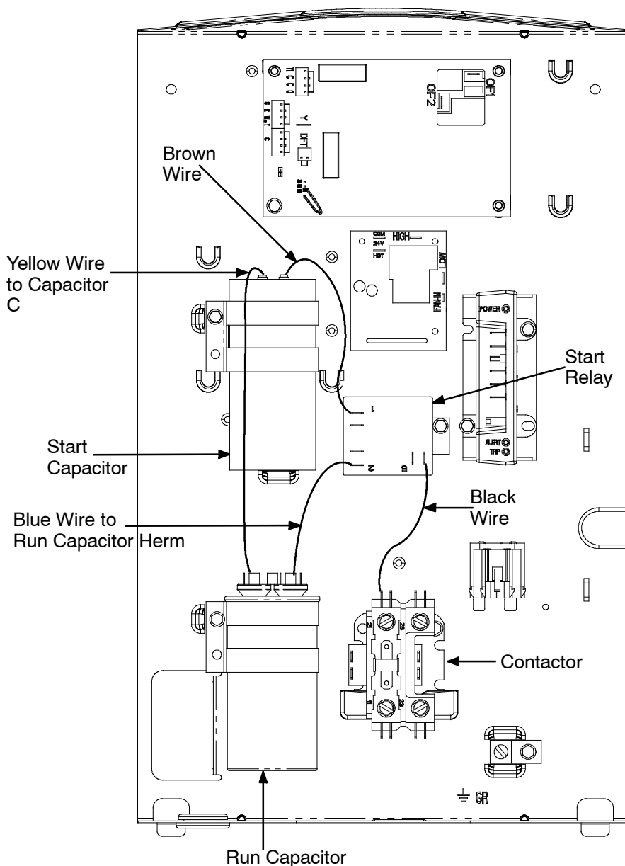
Start Kit Components - Mainline Models, AC & HP: Non-Communicating
