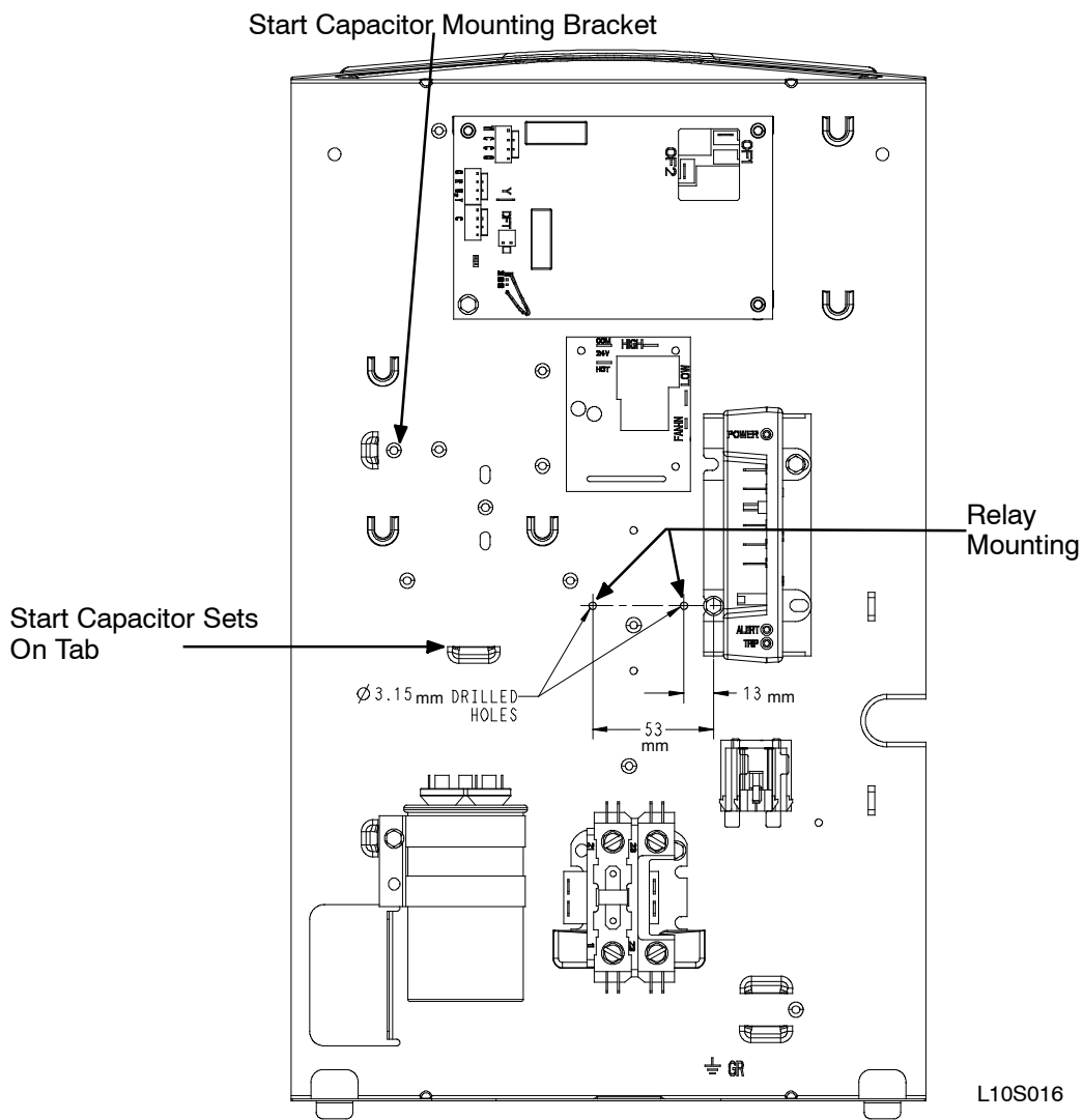
Start Relay & Start Capacitor Mounting Locations - Mainline Models, AC & HP: Non-Communicating
