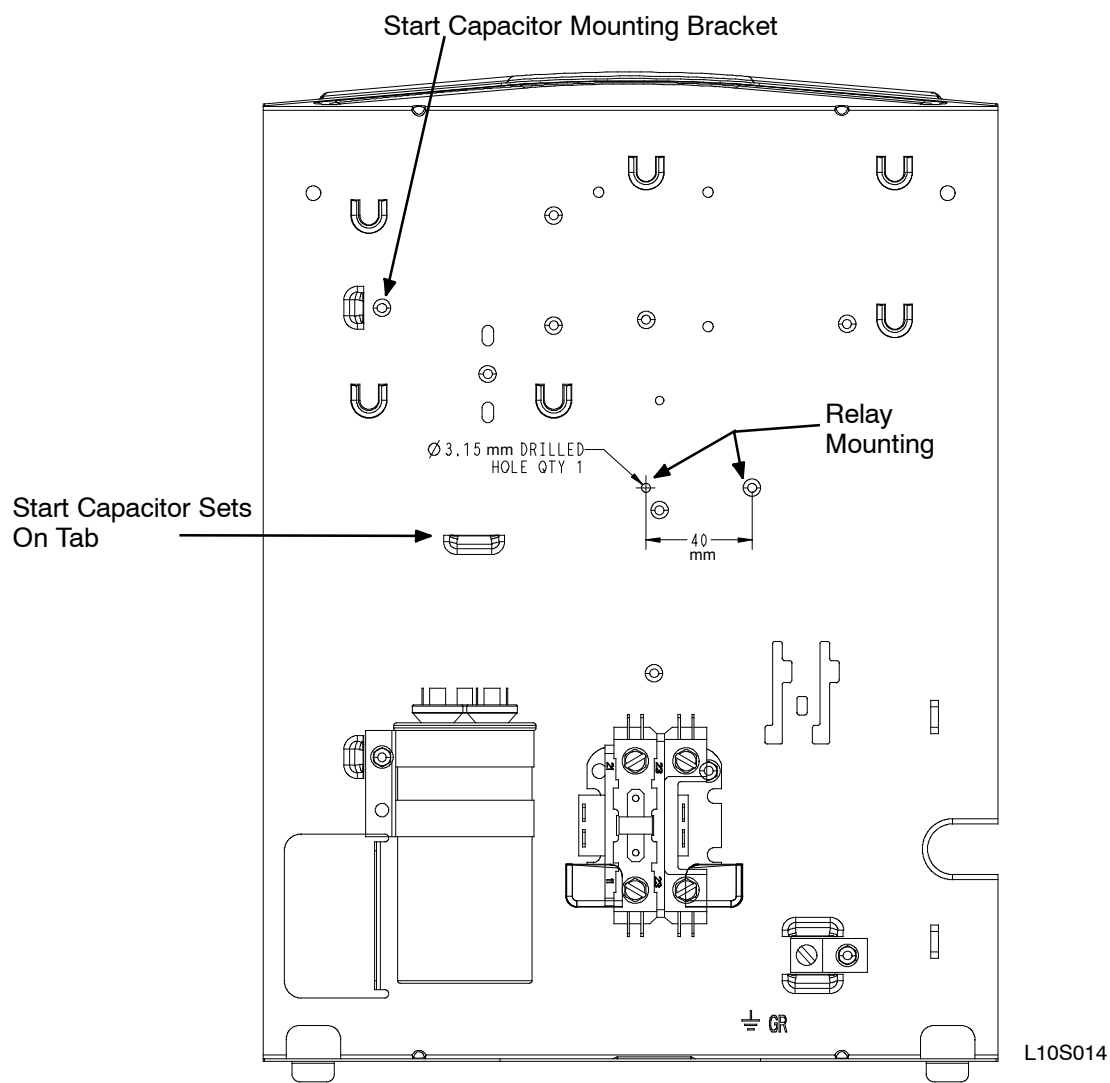
Start Relay & Start Capacitor Mounting Locations - Entry Models, AC & HP
