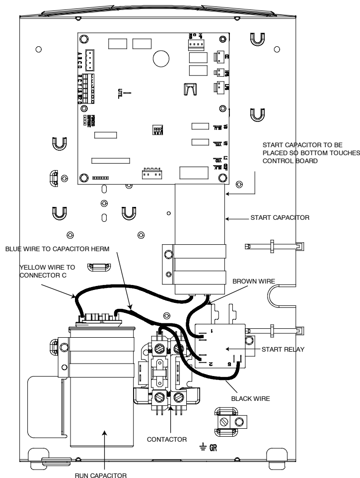
Start Kit Components - Mainline Models, AC & HP: Communicating
