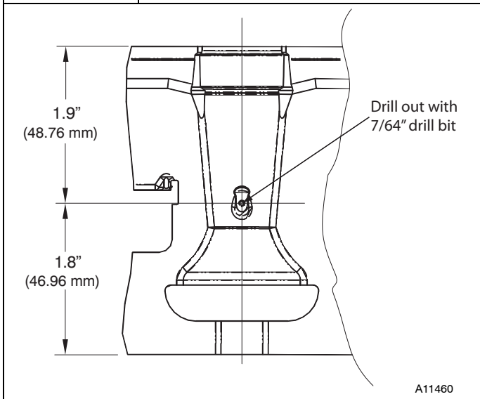
Figure 6 Mixer Screw Location
