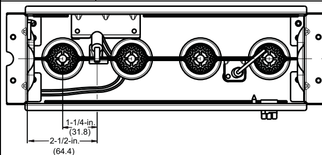
Figure 8 Igniter Position – Side View
