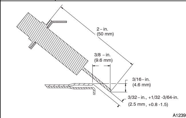
Figure 8 Igniter Position – Side View
