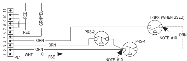
Figure 11 – Pressure Switch Wiring
