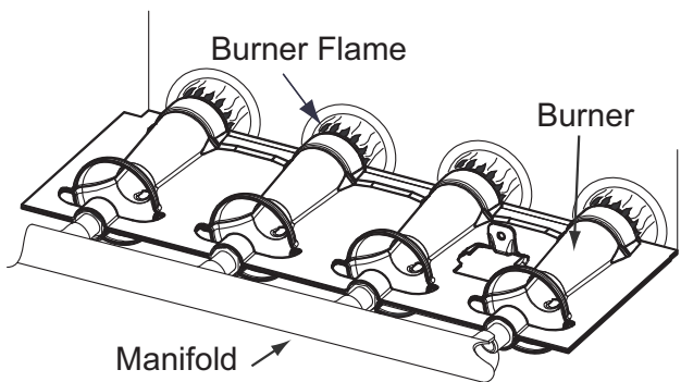
Figure 13 – Burner Flame
