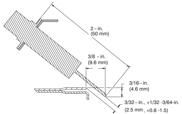
Figure 8 – Igniter Position – Side View
