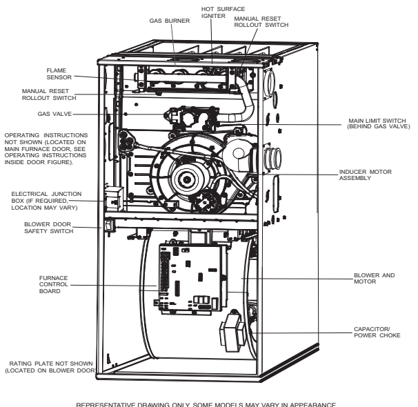
Figure 1 – Representative Furnace Drawing
