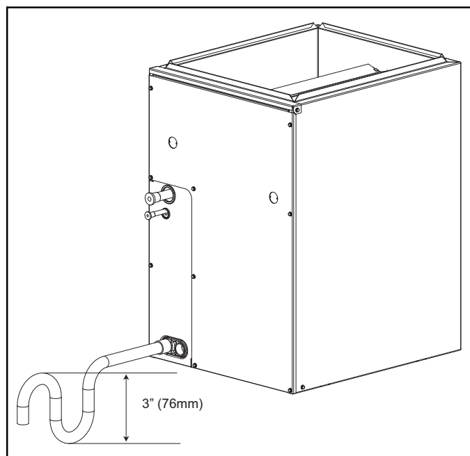
Figure 9 – Condensate Trap
