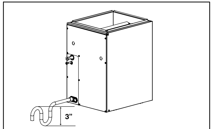
Figure 8 – Condensate Trap
