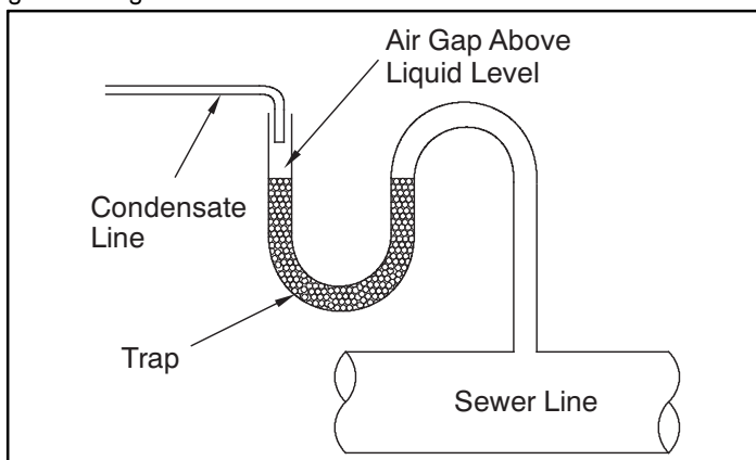
Figure 5 – Condensate Drain to Waste Line
