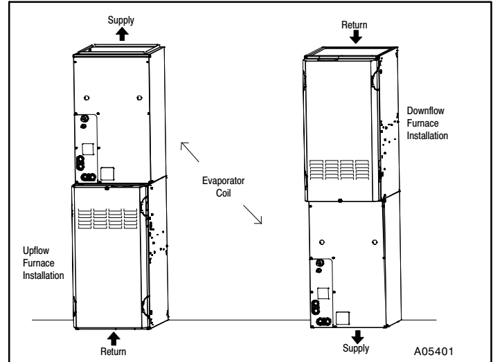
Figure 1 – Correct Orientation of Coil Support on Furnace
