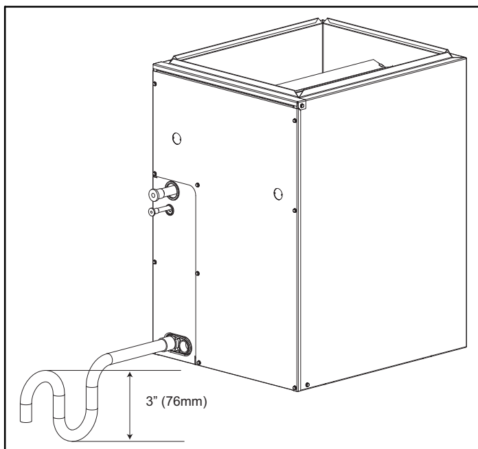
Figure 4 – Condensate Trap
