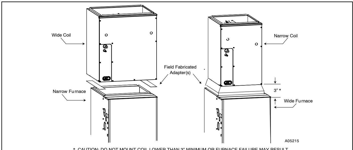
Figure 2 – Adapter(s) Installation When Coil Overhangs or Underhangs Furnace
