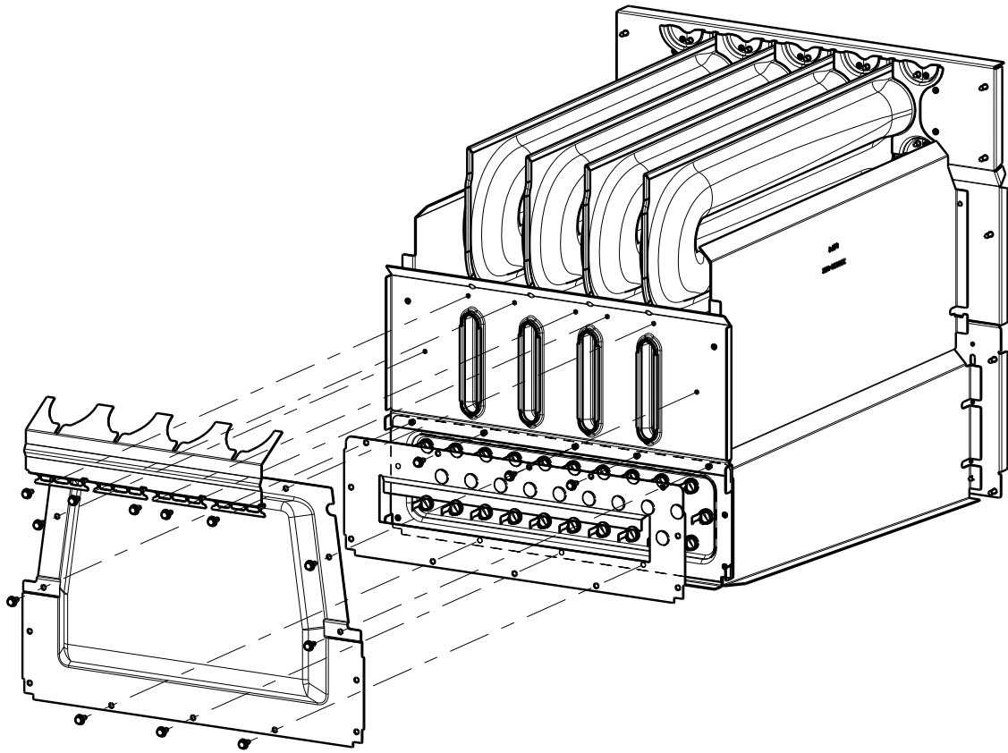
Sidewall Baffle Removal / Installation – Rear View
