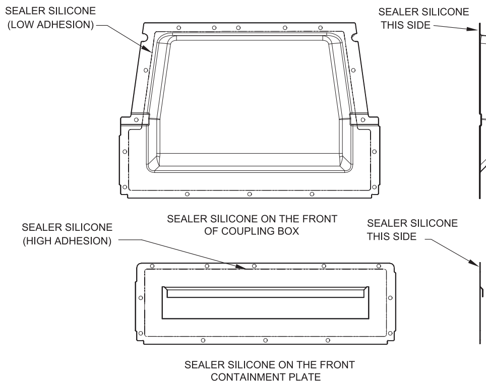
Figure 10 Containment Plate and Collector Box Sealant Application
