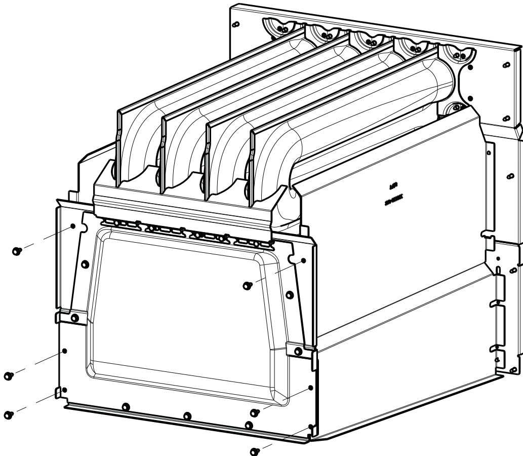
Sidewall Baffle Removal / Installation – Rear View
