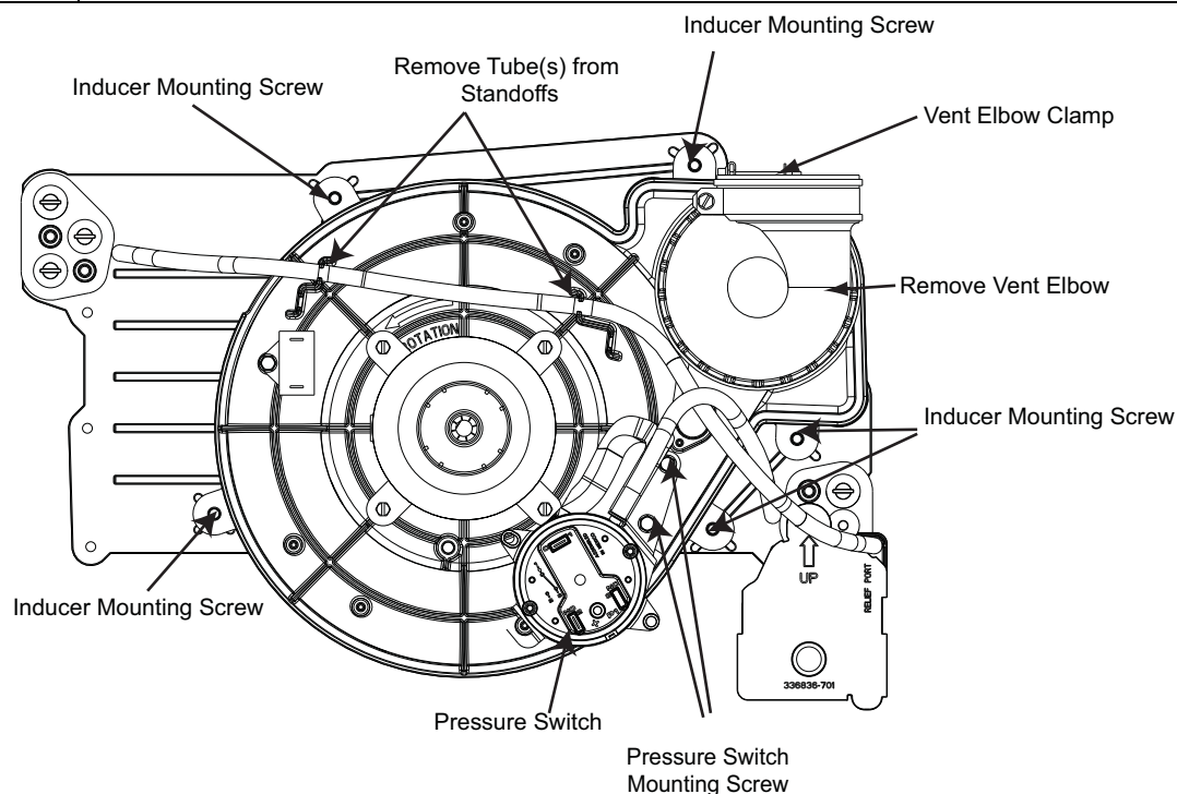
Inducer Assembly Motor (Inducer Motor Fan Subject to Change)
