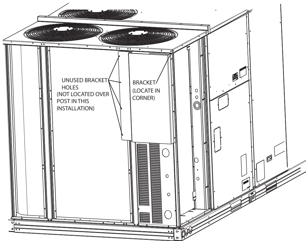
Fig. 2 - Installed Bracket
