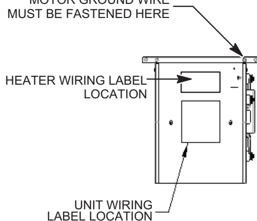
Fig. 2 – Motor Ground and Wire Label Location
