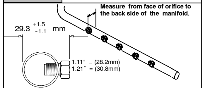
Figure 3 Changing Orifices
