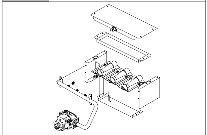
Figure 1 Disassembly
