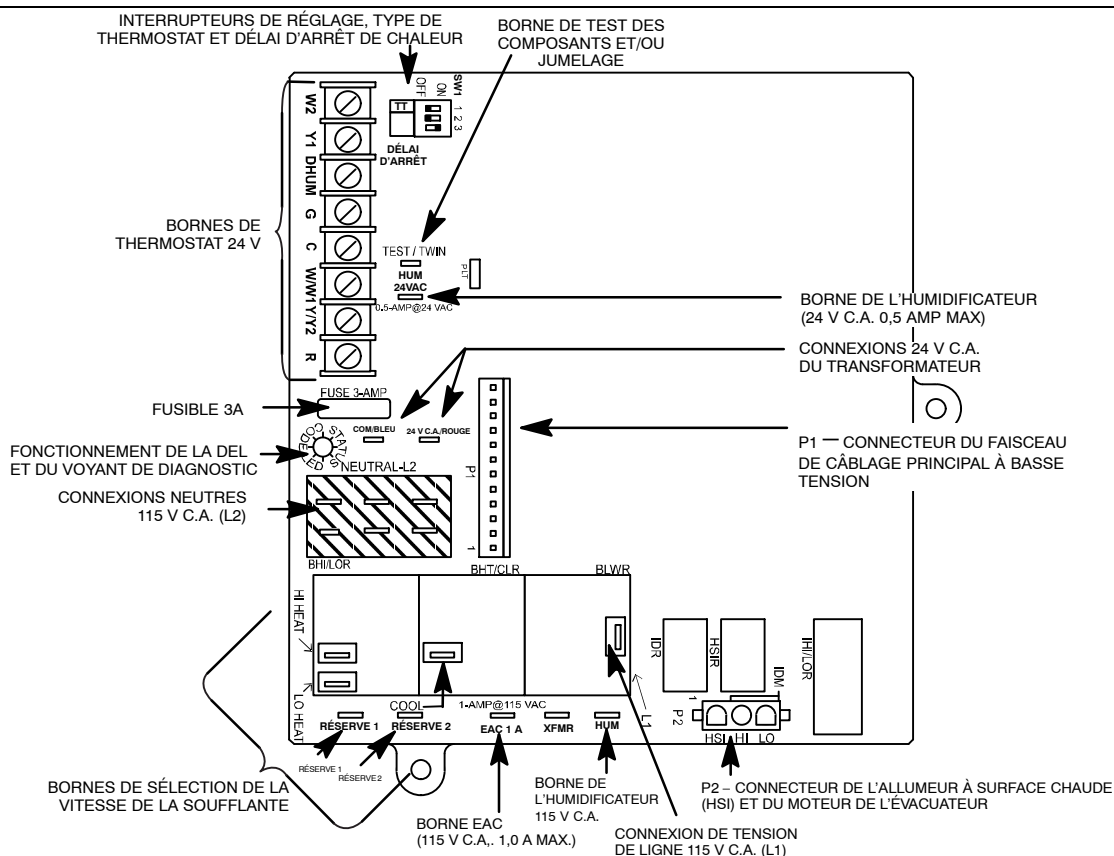
Figure 34 (suite) – Commande de chaudière – 80 %
