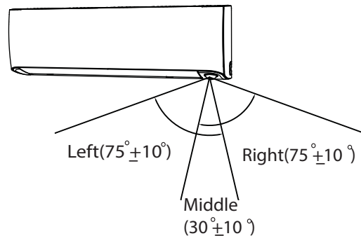
Fig. 18 – Intelligent Eye
