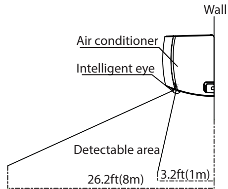
Fig. 17 – Intelligent Eye
