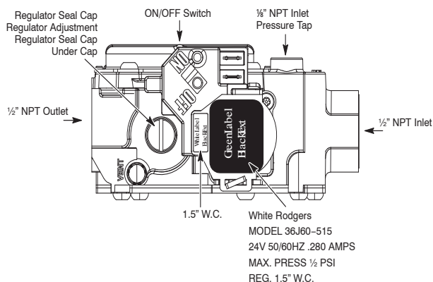
Figure 9 – Low Capacity 26,000 BTUH Gas Valve
