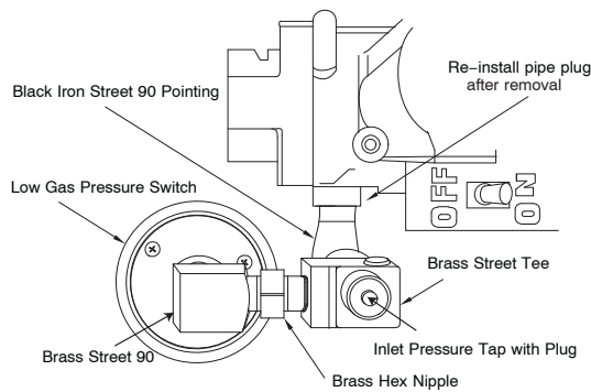
Figure 10 – Low Gas Pressure Switch – All Widths
