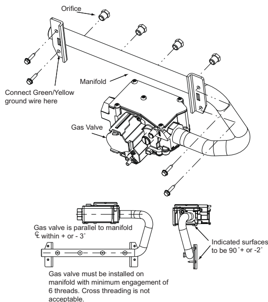
Figure 2 – Manifold Assembly
