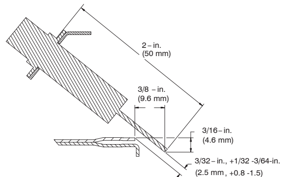
Figure 9 Igniter Position – Side View
