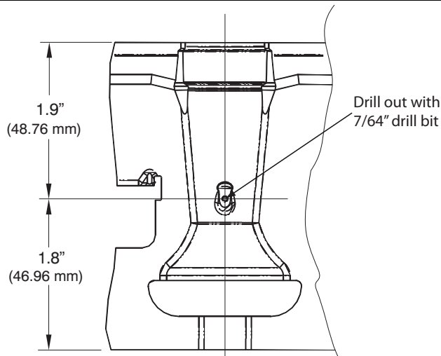
Figure 7 Mixer Screw Location
