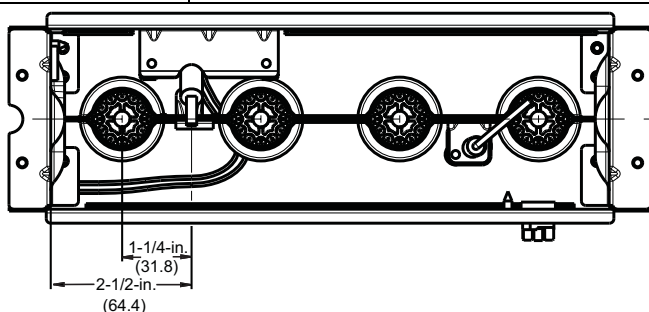
Figure 8 Igniter Position – Top View
