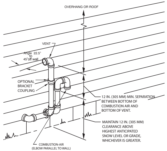
Figure 46 Vent Terminations
