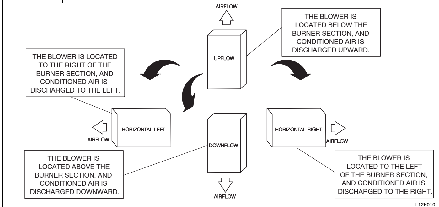
Figure 3 Multipoise Orientations
