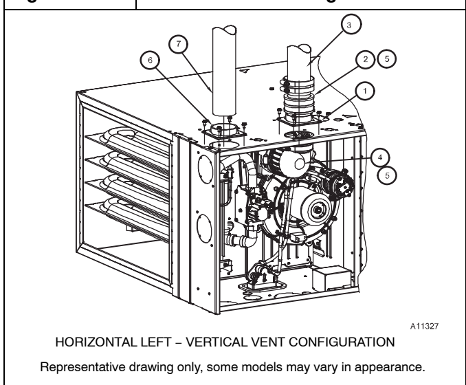
Figure 53 Horizontal Left Configurations
