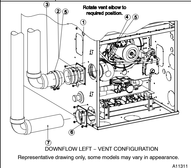
Figure 52 Downflow Configurations
