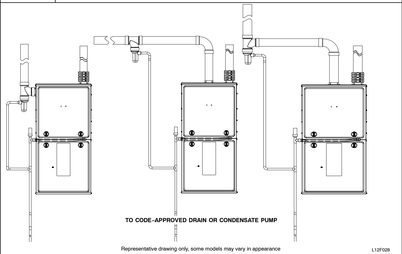
Figure 49 Optional Combustion Air Inlet Moisture Trap
