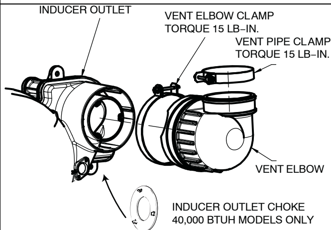
PSC INDUCER ASSEMBLY
