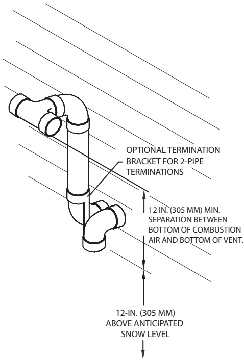
Figure 44 Tee at Termination Outlet
