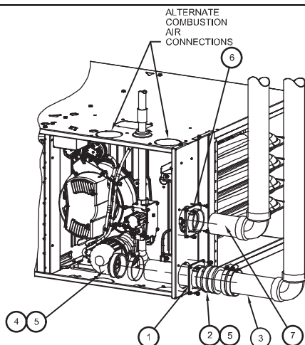
HORIZONTAL RIGHT - RIGHT VENT CONFIGURATION A11335 Representative drawing only, some models may vary in appearance.
