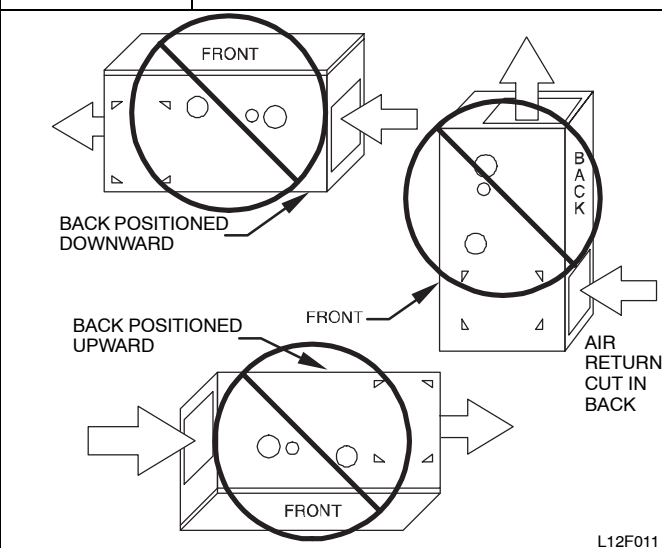
Figure 5 Prohibit Installations
