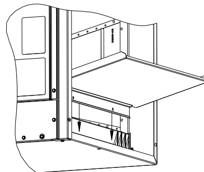
Figure 3 – Horizontal–Right Installation of Pan Extension (43, 60, & 61 sizes only)
