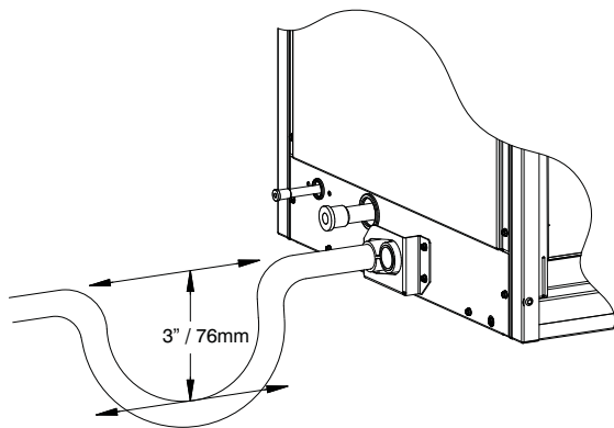
Figure 8 – Condensate Trap
