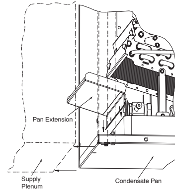
Figure 2 – Horizontal–Left Installation of Pan Extension (43, 60, & 61 sizes only)
