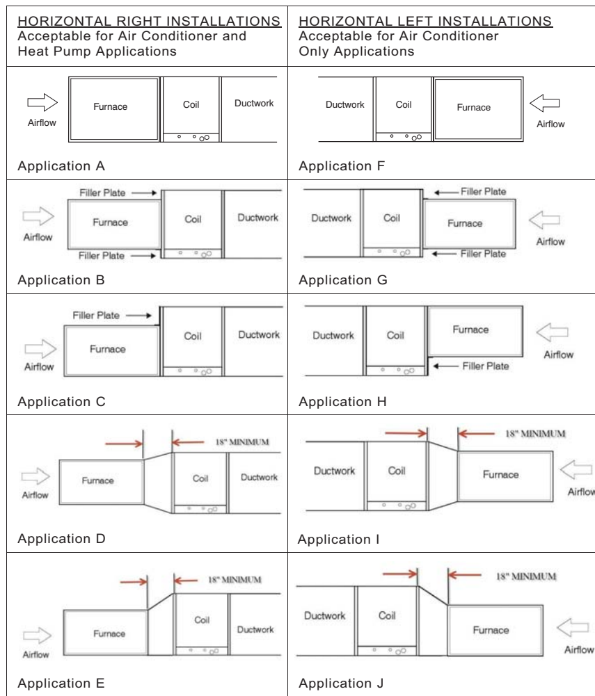
Figure 4 – Horizontal Installation Applications
