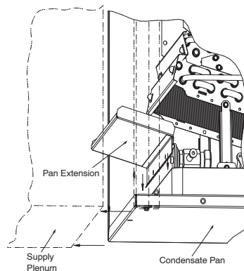
Figure 4 - Horizontal-Left Installation of Pan Extension
