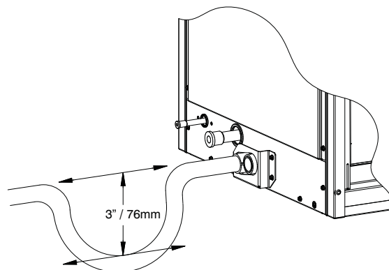
Figure 9 - Condensate Trap
