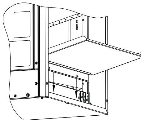
Figure 5 - Horizontal-Right Installation of Pan Extension
